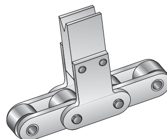
Fig. 15 SK Attachments with V-block
