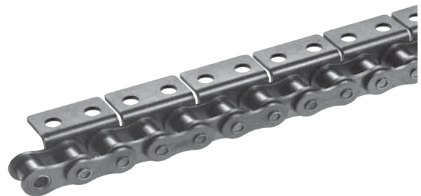
Fig. 2 Single Pitch Attachment Chain
