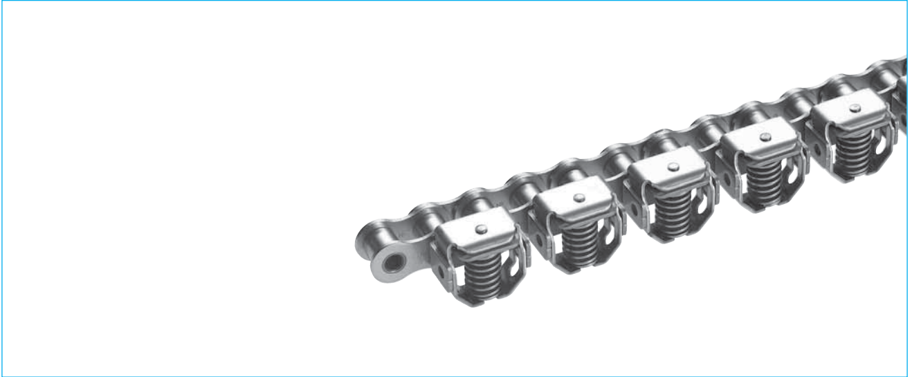
Fig. 29 RS08B and RS10B Gripper Chain
