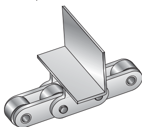
Fig. 11 K Attachment with L-angle
