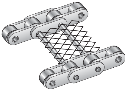
Fig. 7 Cross rods with mesh
