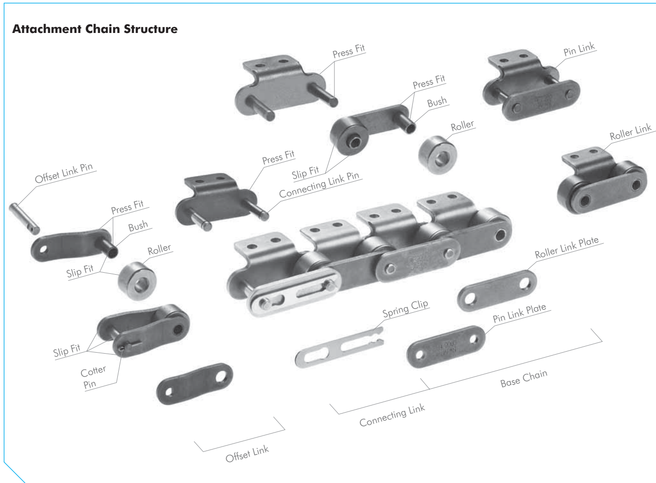
Fig. 1 Basic Attachment Chain Structure
